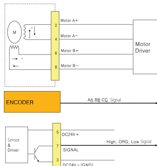
System Configuration Diagram
