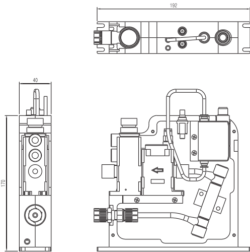
LO Serise Dimension drawing
